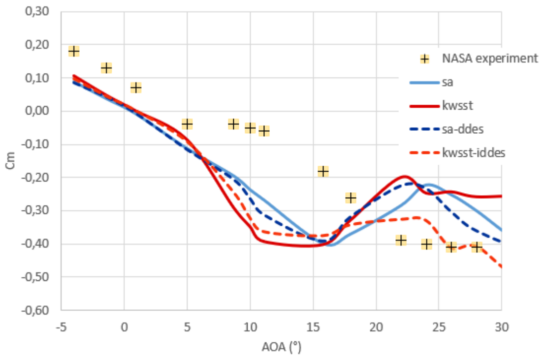
Figure 83: Pitching moment coefficient w.r.t angle of attack.
