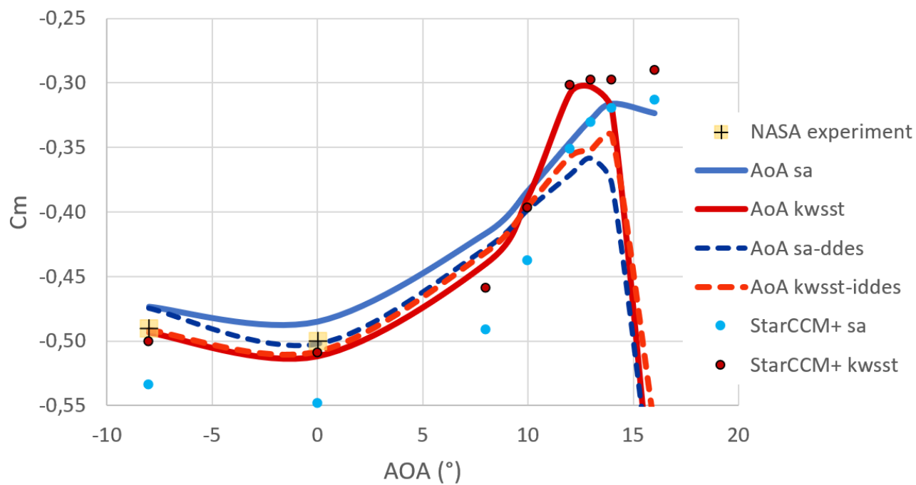
Figure 70: Pitching coefficient w.r.t angle of attack.
