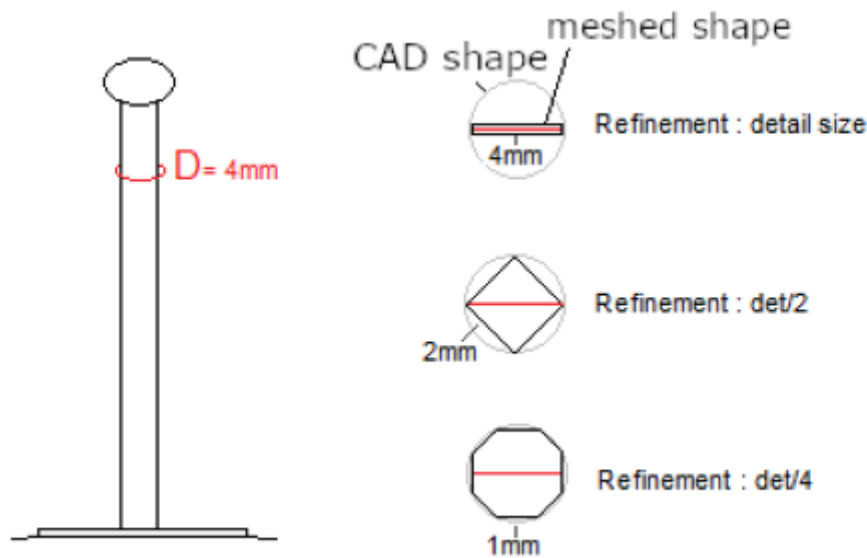
Figure 55: Aircraft antenna.
