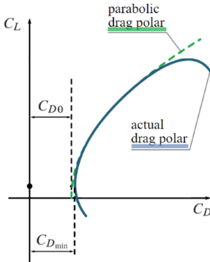
Figure 25: Parabolic drag and actual drag polar.
