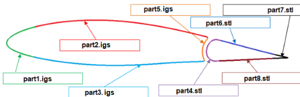
Figure 51: Closed volume composed of mutiple parts.
