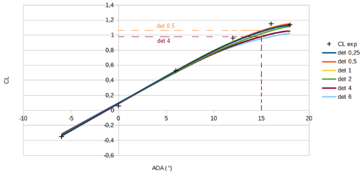
Figure 49: CL w.r.t AoA (different detail sizes).
