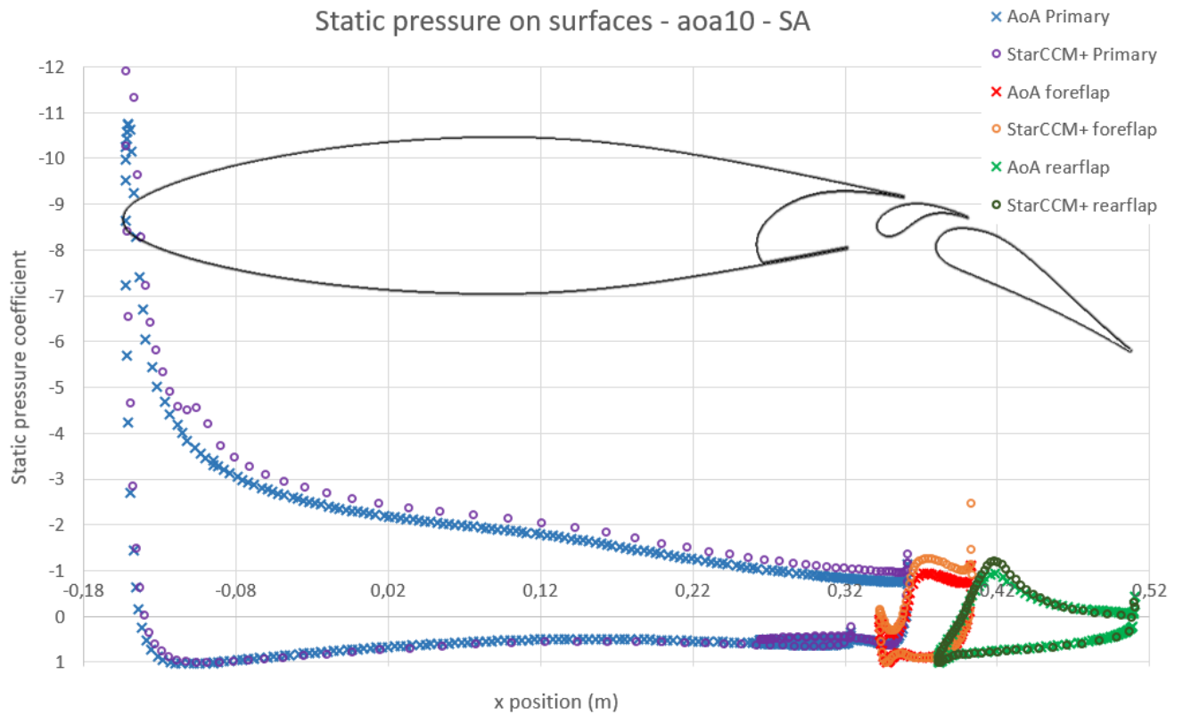
Figure 74: Comparison of static pressure values at 10^\circ of angle of attack using the Spalart-Allmaras turbulence model, for Ace of Aircraft and StarCCM+.
