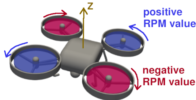
Figure 47: Rotor direction when main orientation is Z.
