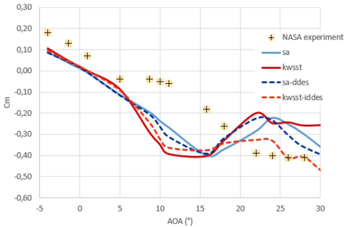
Figure 85: Pitching moment coefficient w.r.t angle of attack.
