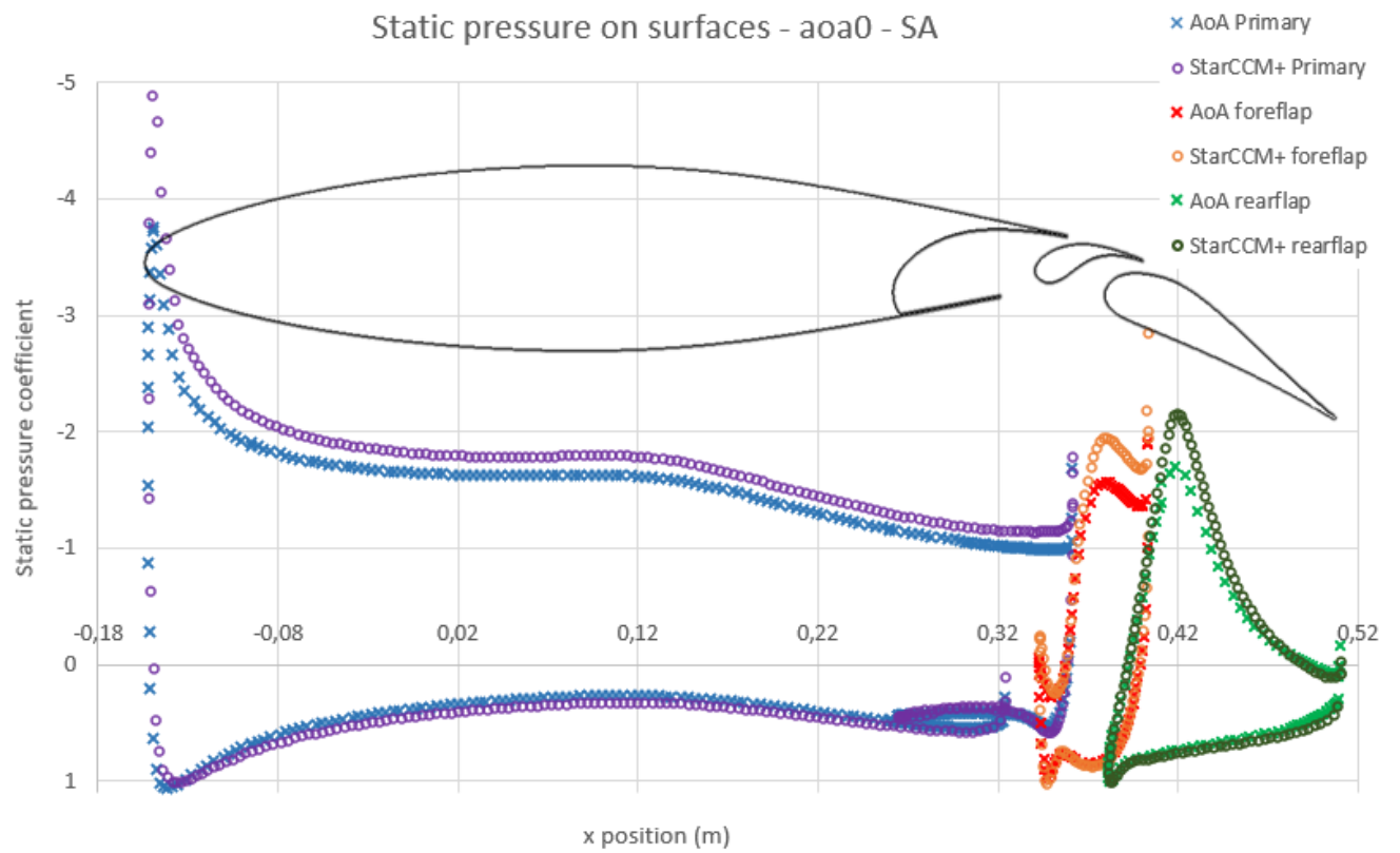
Figure 74: Comparison of static pressure values at 0° of angle of attack using the Spalart-Allmaras turbulence model, for Ace of Aircraft and StarCCM+.
