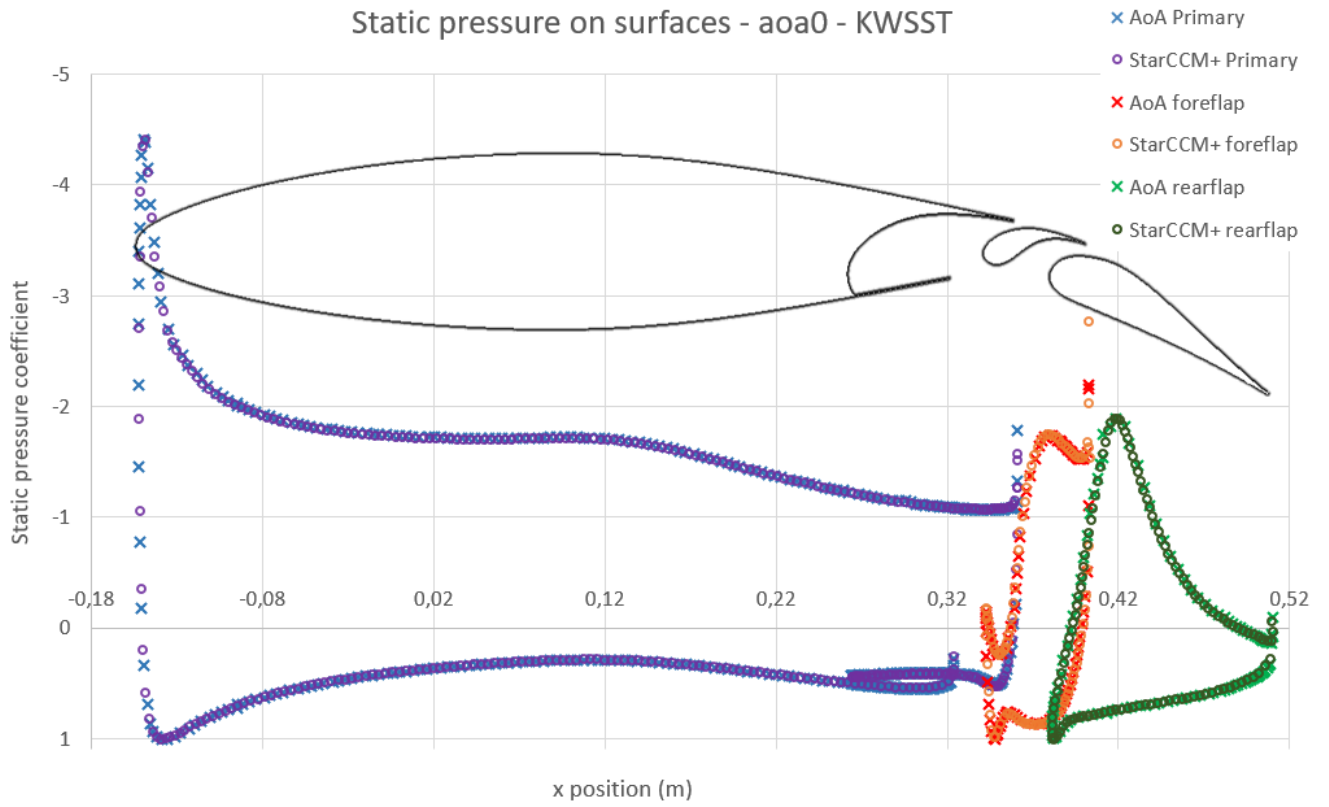
Figure 73: Comparison of static pressure values at 0^\circ of angle of attack using the k-omega SST turbulence model, for Ace of Aircraft and StarCCM+.
